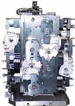
FOUR SIDED TOMBSTONE FIXTURE FOR 300 MM PALLET
